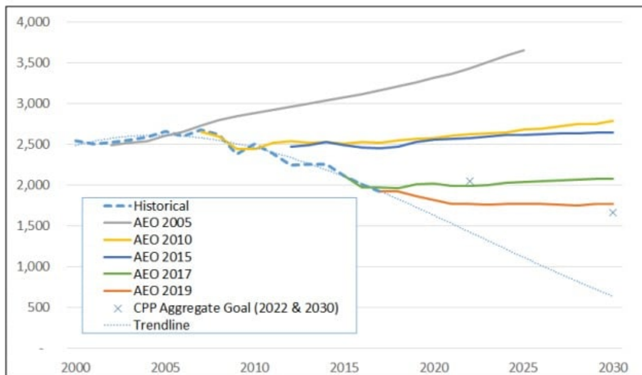
Figure 2-7 Power Sector CO 2 Emissions (million short tons)
